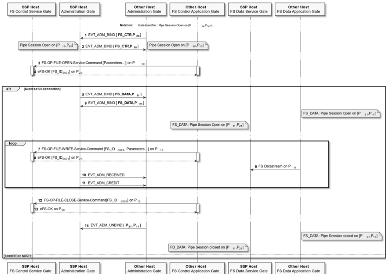
Figure G.3: File writing from data stream
